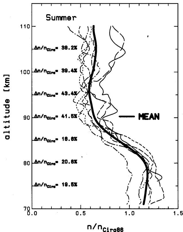
Fig. 8. All summer density profiles measured with the TOTAL or CONE ionization gauges divided by the appropriate CIRA86 reference profile. The thick line indicates the mean profile of all ionization gauge measurements. Furthermore, the deviation between the mean ionization gauge densities and CIRA86 is indicated every 5 km.
