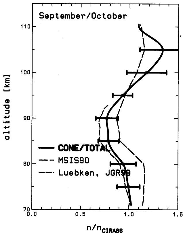
Fig. 10. As for Fig. 9 but for the months September and October.
