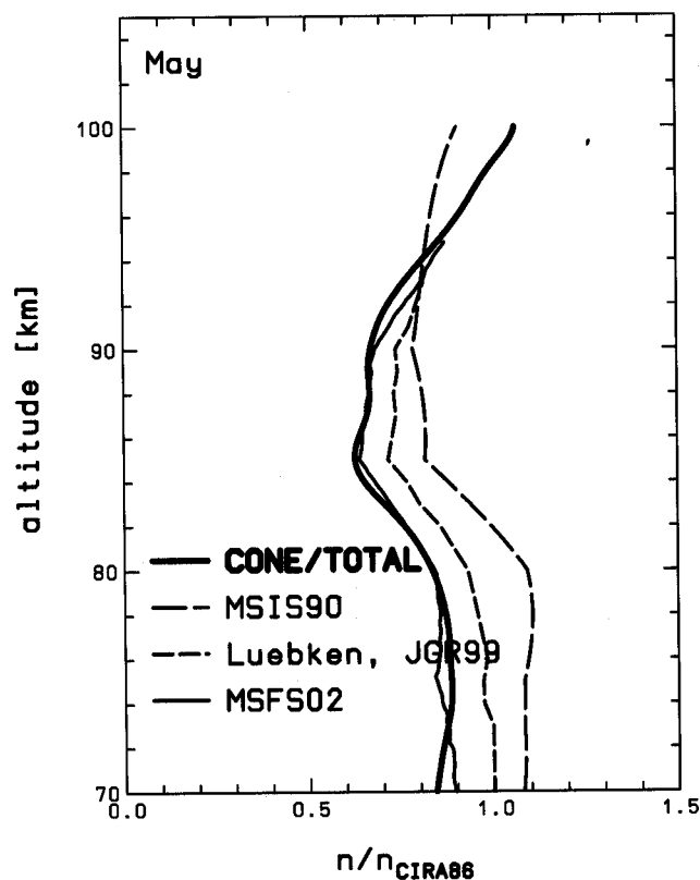
Fig. 12. As for Fig. 9 but for May. The ionization gauge data set comprises only of a single rocket flight in this case. For comparison we also show the data of a falling sphere, labeled MSFS02, measured only a few minutes before the sounding rocket flight.
