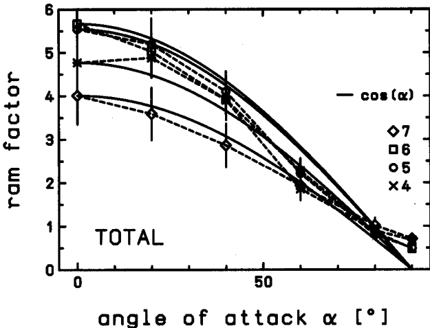
Fig. 3. As for Fig. 2 but for TOTAL.
