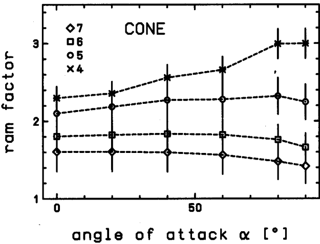
Fig. 2. Ram-factors for CONE as a function of the angle of attack measured for different flow conditions. The different results are labeled according to the flow condition number given in Table 3.
