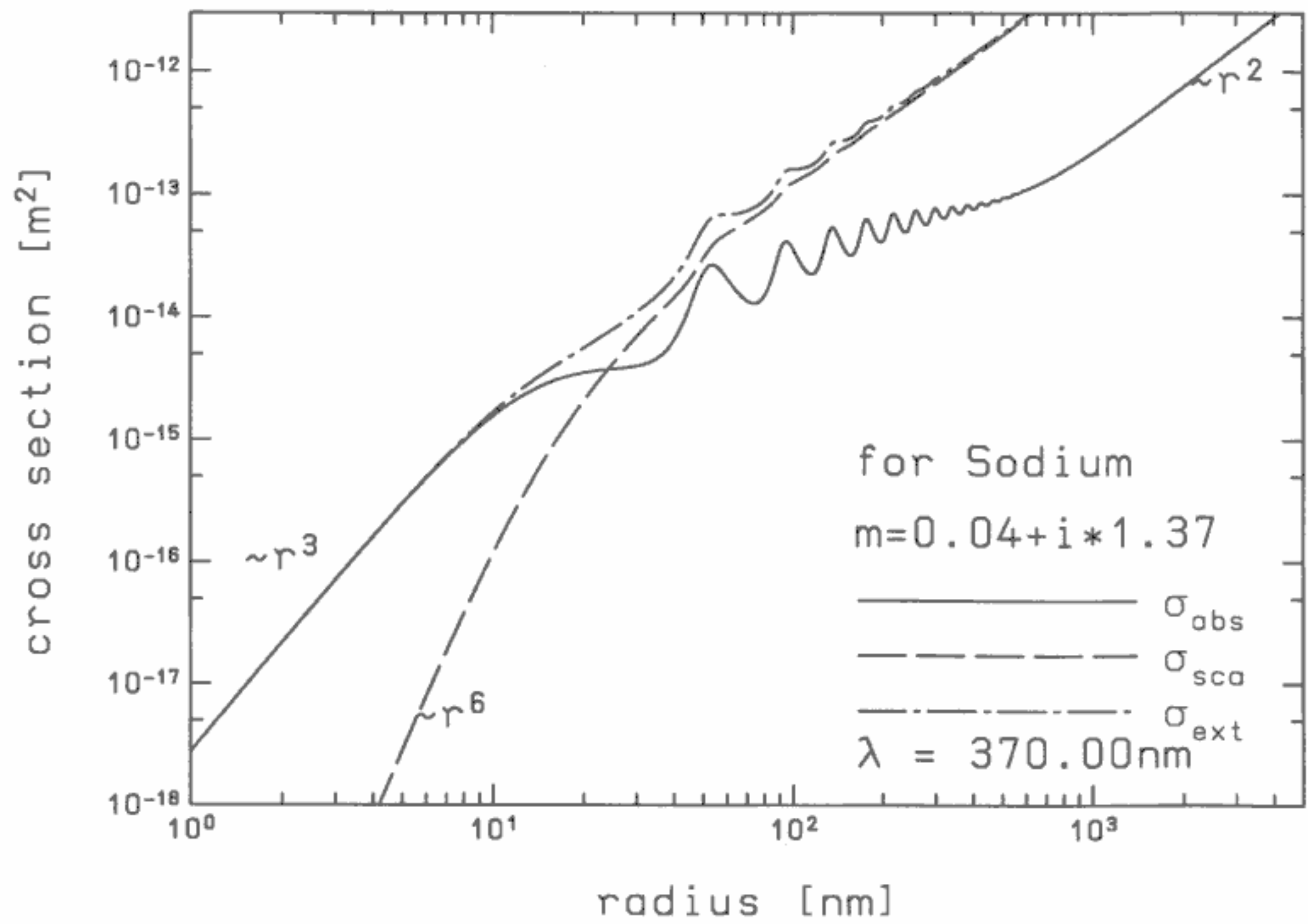
Fig. 3. Radial dependences of Mie cross sections for absorption, scattering, and extinction as a function of particle radius for a wavelength of 370 nm. For particles smaller than ~10 nm the absorption cross section is proportional to the volume of the particle, and for particles larger than 1000 nm it is proportional to its surface. In between, there is a smooth transition with an approximate r^1 dependence and interference patterns overlayed.
